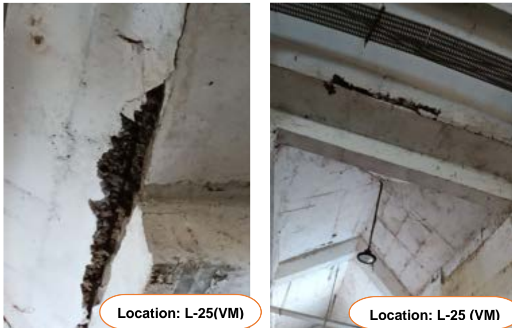
Fig. 8.3: Spalling of Concrete & Loss of Reinforcement
